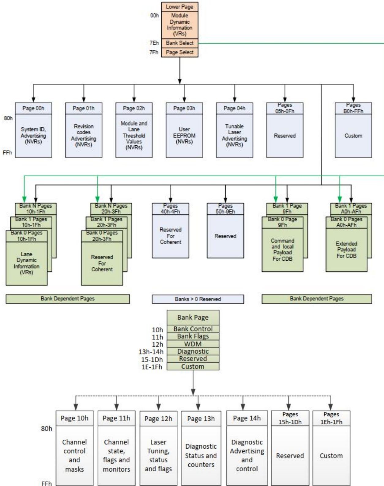
Figure 2. SFP112 Memory Map
