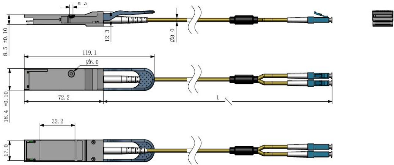
Figure 9. Mechanical Specifications
